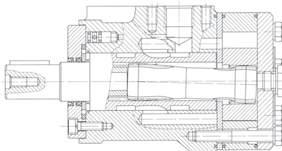
(1)EPMZM、EPMZ、EPMZR、EPMZ1、EPMZH、EPMZ2 & EPMZ3 series with axial oil distribution structure.
