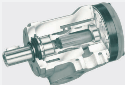
(1)EPMZM、EPMZ、EPMZR、EPMZ1、EPMZH、EPMZ2 & EPMZ3 series with axial oil distribution structure.
