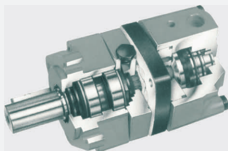
(2)EPMZSY、EPMZT & EPMZV series with Disc oil distribution structure.
