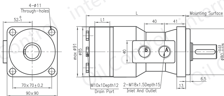
I4: Four Hole Square—flange
