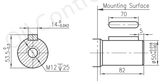
Parallel Key Shaft: B2 Parallel Key : 14X9X70
