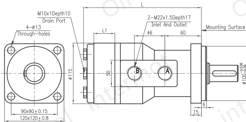
I4: Four Hole Square-flange
