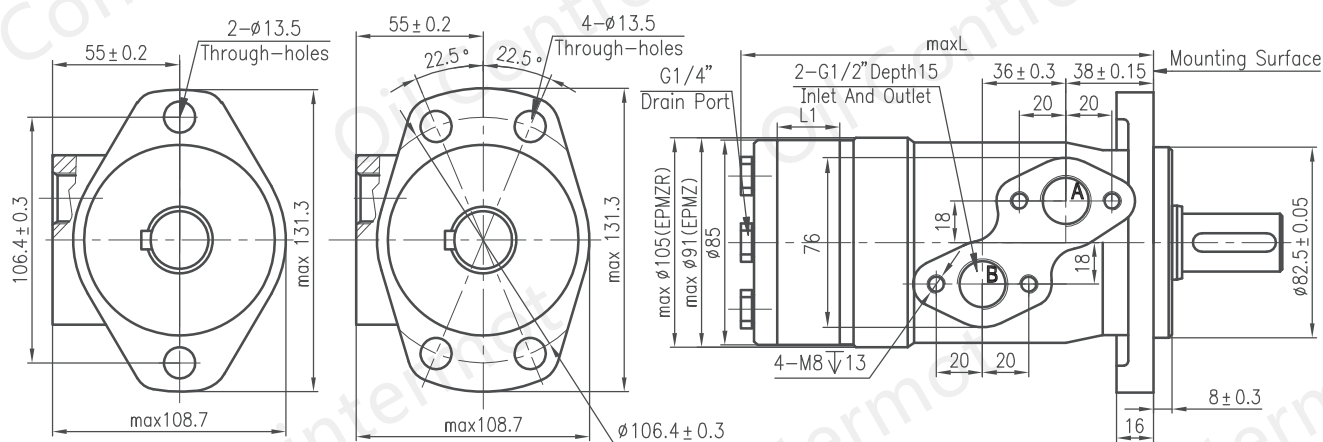
I: Two Hole Rhomb-flange
