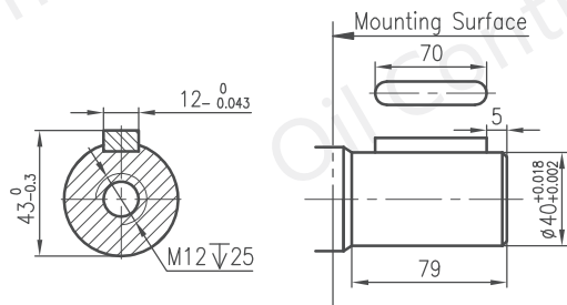
Standard Parallel Key Shaft: B1 Parallel Key : 12X8X70
