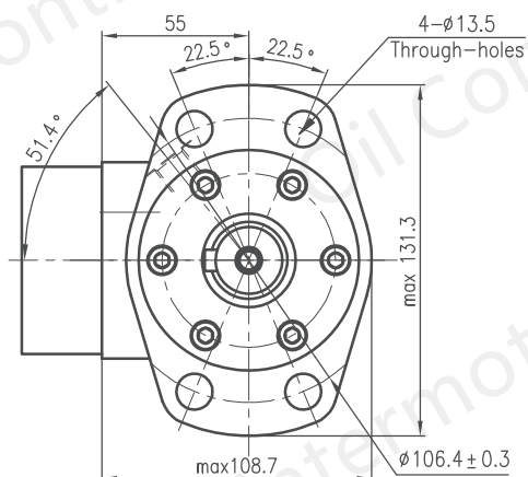
II4: Four Hole Rhomb-flange
